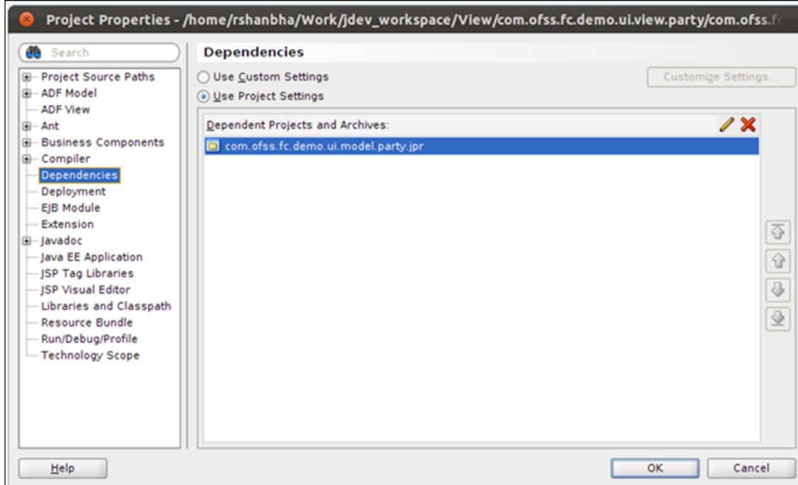
Figure 4–61 Dependencies
