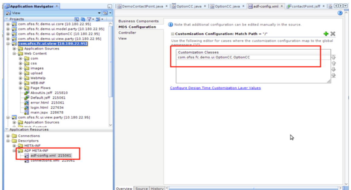
Figure 4–7 Adding com.ofss.fc.demo.ui.OptionCC.OptionCC
