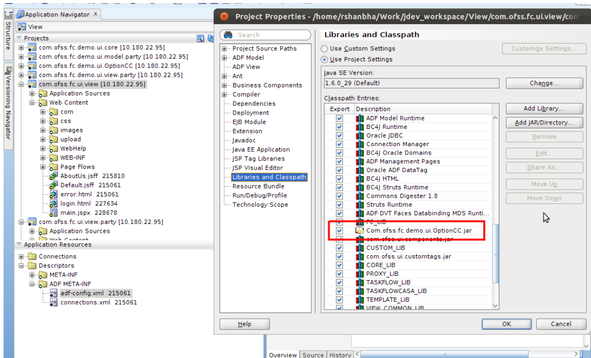
Figure 4–6 Adding com.ofss.fc.demo.ui.OptionCC.jar
